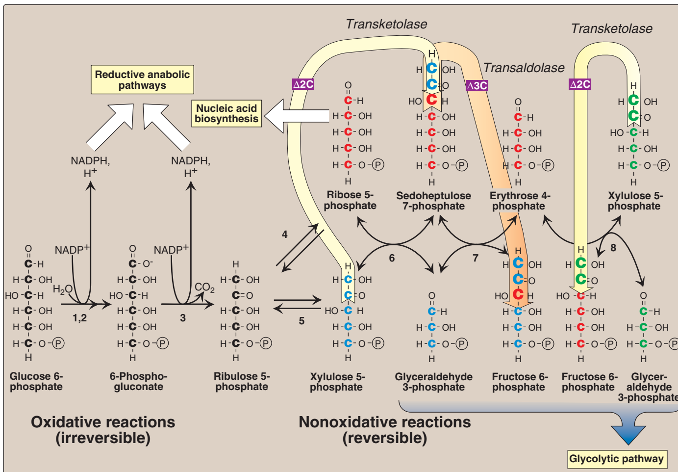
Figure 13.2 Reactions of the hexose monophosphate pathway. Enzymes numbered above are: 1,2) glucose 6-phosphate dehydrogenase and 6-phosphogluconolactone hydrolase , 3) 6-phosphogluconate dehydrogenase , 4) ribose 5-phosphate isomerase , 5) phosphopentose epimerase , 6) and 8) transketolase (coenzyme: thiamine pyrophosphate), and 7) transaldolase . \Delta 2C = two carbons are transferred in transketolase reactions; \Delta 3C = three carbons are transferred in the transaldolase reaction.
