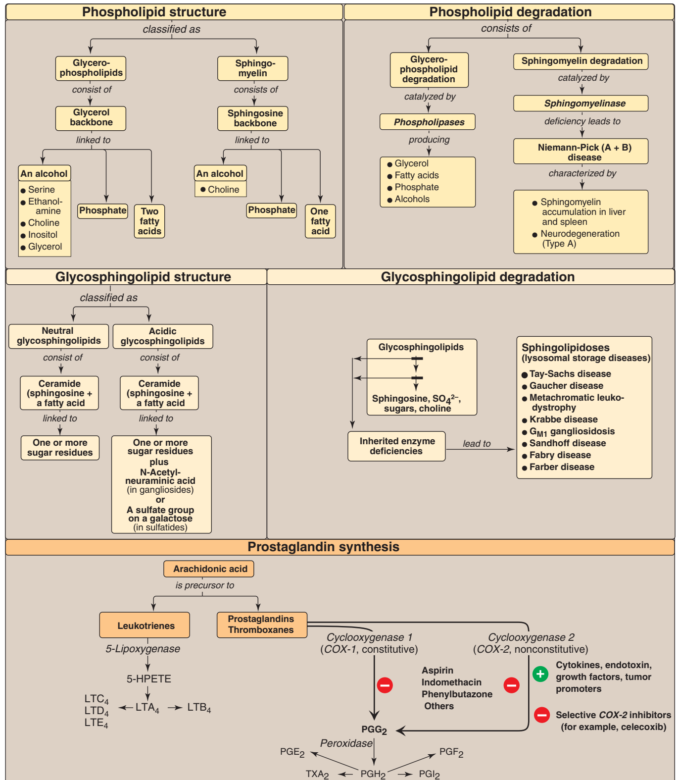
Figure 17.25 Key concept map for complex lipids.
