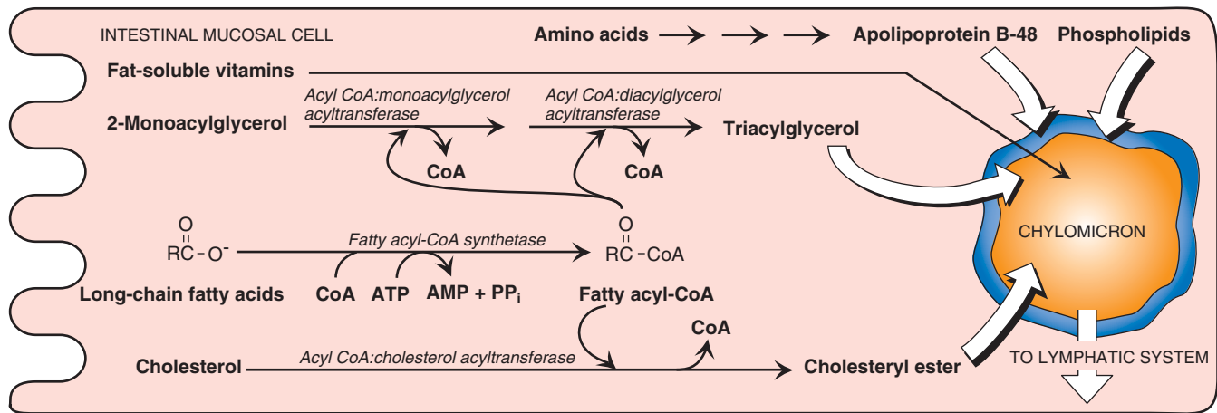
Figure 15.6 Assembly and secretion of chylomicrons by intestinal mucosal cells. [Note: Short- and medium-chain length fatty acids do not require incorporation into micelles and directly enter into the blood.]
