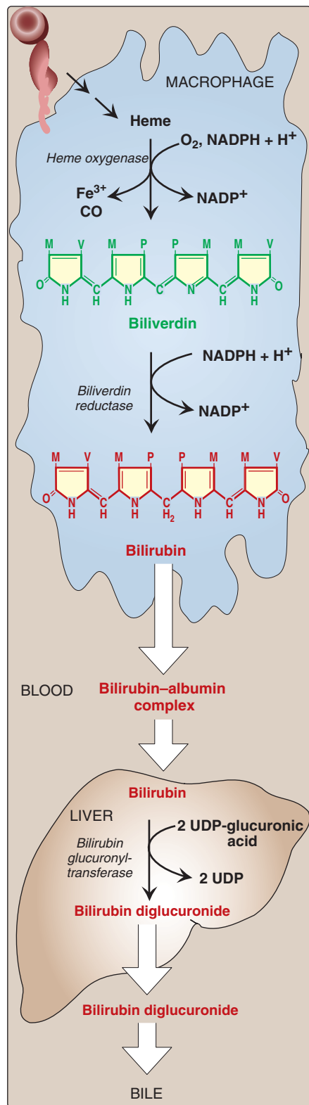
Figure 21.9 Formation of bilirubin from heme. UDP = uridine diphosphate.
