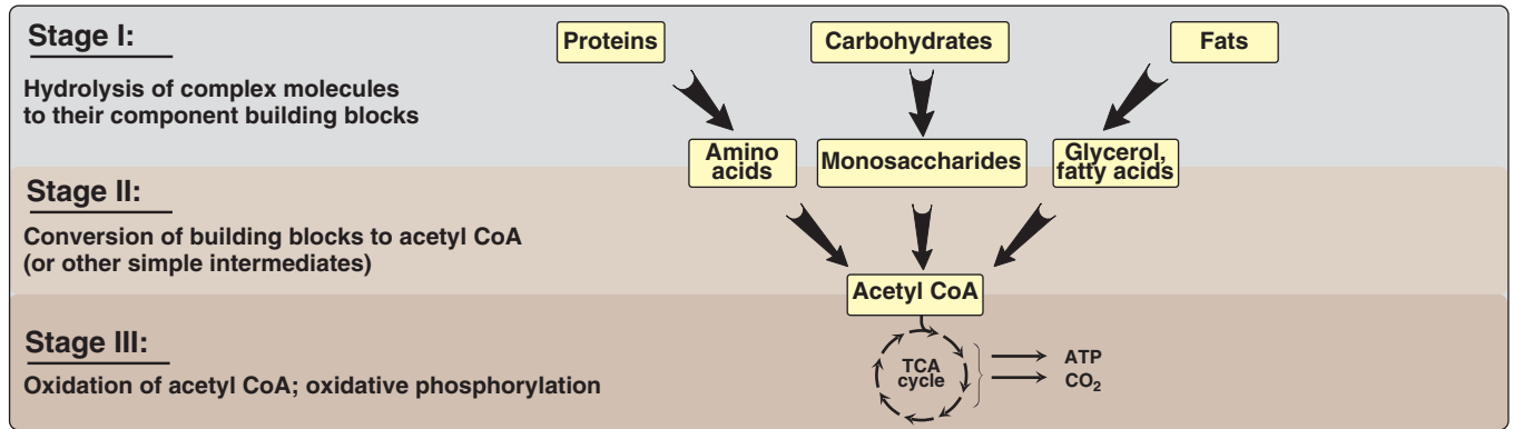
Figure 8.3 Three stages of catabolism.
