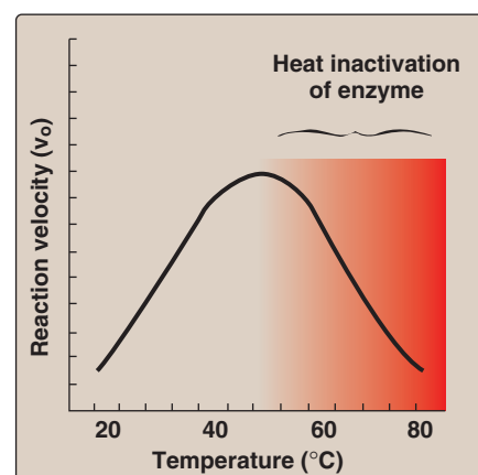
Figure 5.7 Effect of temperature on an enzyme-catalyzed reaction.
