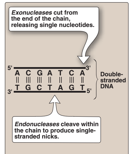
Figure 29.18 Endonuclease versus exonuclease activity.
