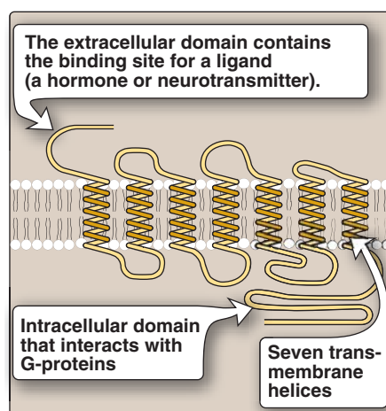
Figure 8.6 Structure of a typical G protein-coupled receptor (GPCR) of the plasma membrane.
