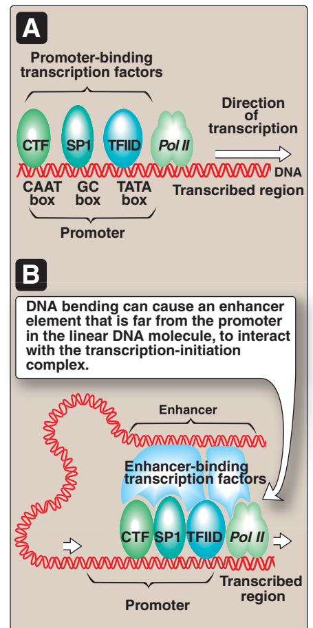
Figure 30.13 A. Eukaryotic general transcription factors (CTF, SP1, TFIID) bind to consensus sequences found in promoters for RNA polymerase II . Additional general transcription factors (TFIIs) are required for assembly of the initiation complex and recruitment of polymerase. B. Enhancer stimulation of RNA polymerase II .
