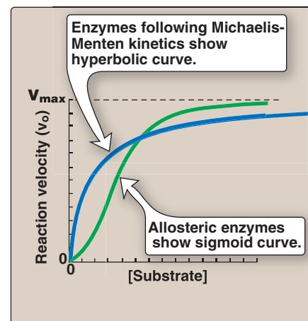
Figure 5.6 Effect of substrate concentration on reaction velocity.
