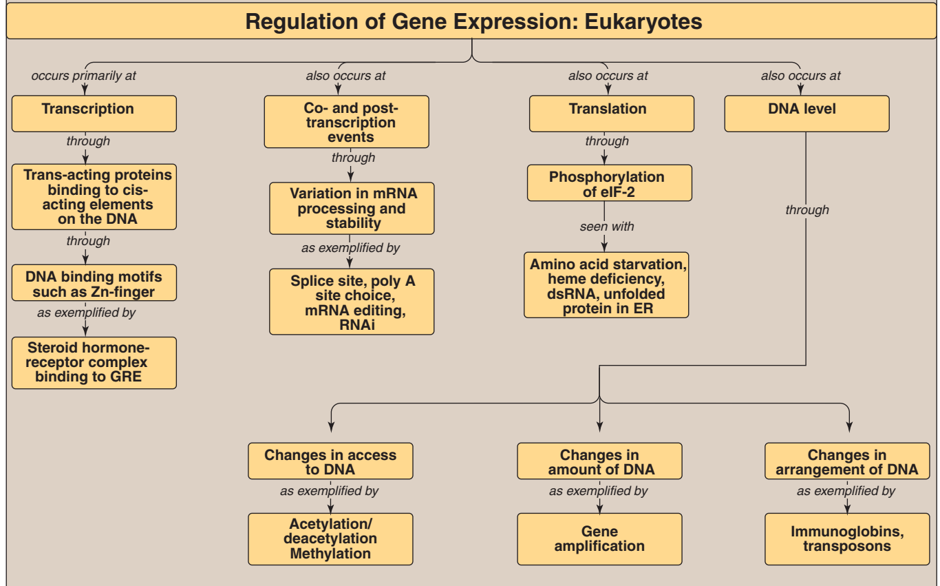
Figure 32.19 Summary of key concepts for the regulation of gene expression.
