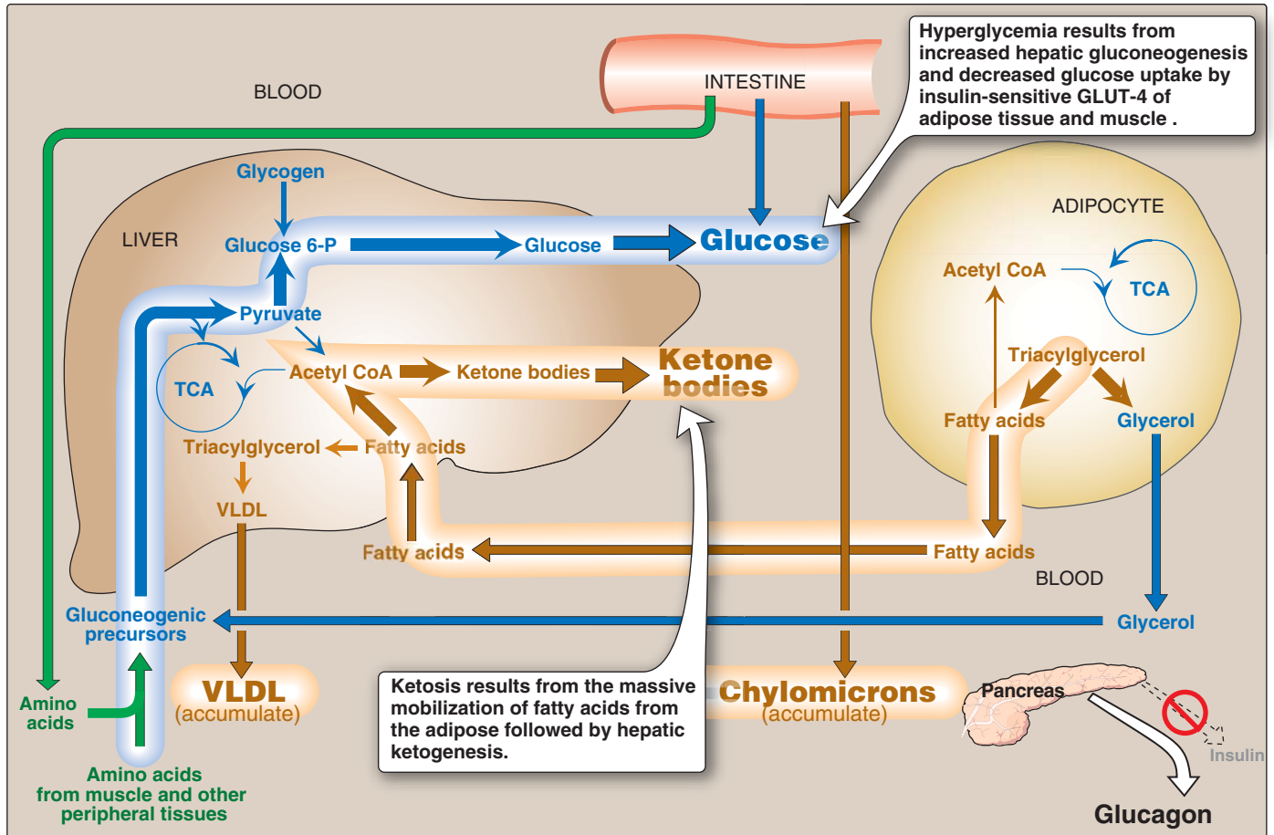
Figure 25.3 Intertissue relationships in type 1 diabetes.
