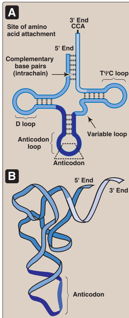
Figure 30.3 A. Characteristic tRNA secondary structure. B. Folded (tertiary) tRNA structure found in cells. D = dihydrouracil. Ψ = pseudouracil.
