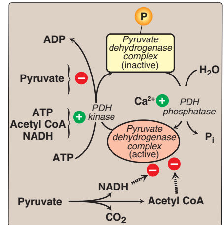
Figure 9.3 Regulation of pyruvate dehydrogenase complex . [-----> denotes product inhibition.]
