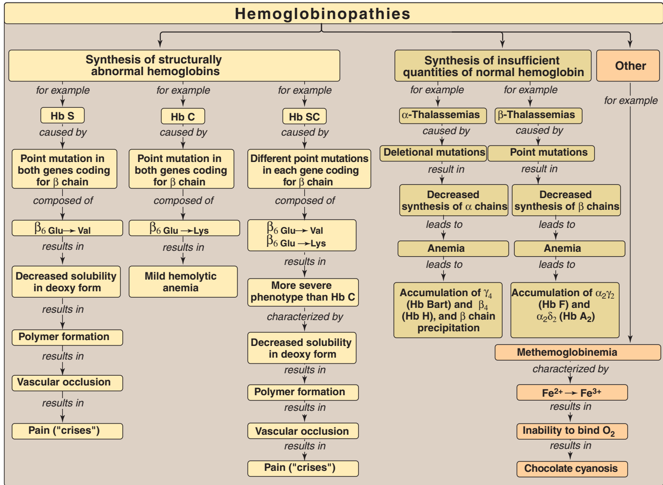
Figure 3.25 Key concept map for hemoglobinopathies.
