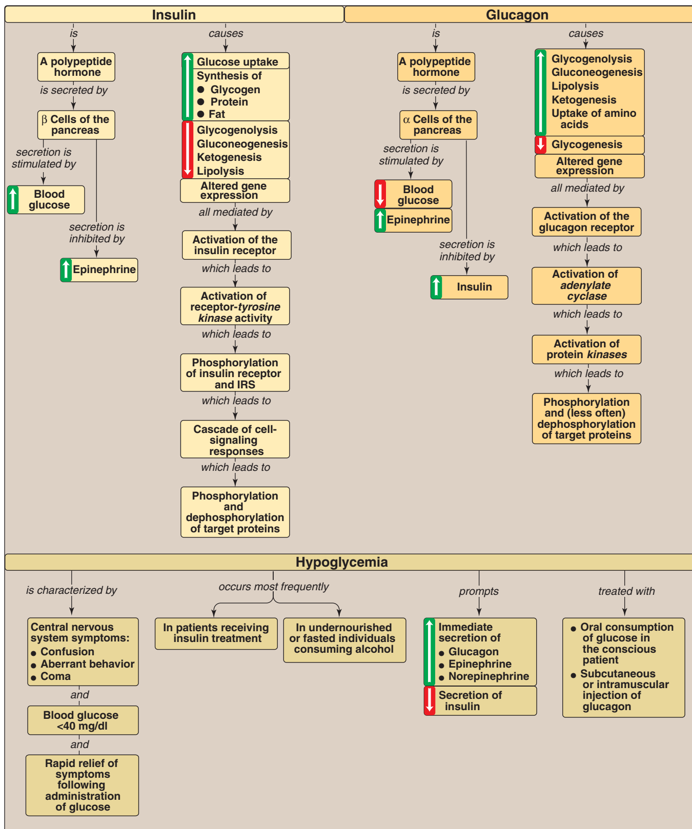
Figure 23.17 Key concept map for integration of energy metabolism.
