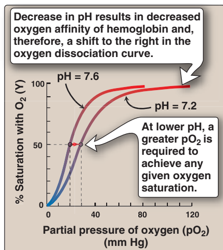
Figure 3.8 Effect of pH on the oxygen affinity of hemoglobin. Protons are allosteric effectors of hemoglobin.
