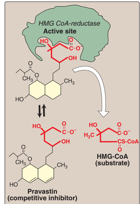
Figure 5.13 Pravastatin competes with HMG-CoA for the active site of HMG-CoA reductase .
